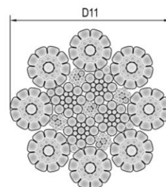
Wire rope cross section 8×26, Wire Strength 2160 N/mm²
