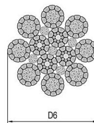
Wire rope cross section 8x26, Wire Strength 2160 N/mm²
