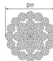
Wire rope cross section 35x7, Wire Strength 2160 N/mm² (Hol.≥24)
