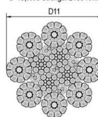
Wire rope cross section 8×19, Wire Strength 2160 N/mm²
